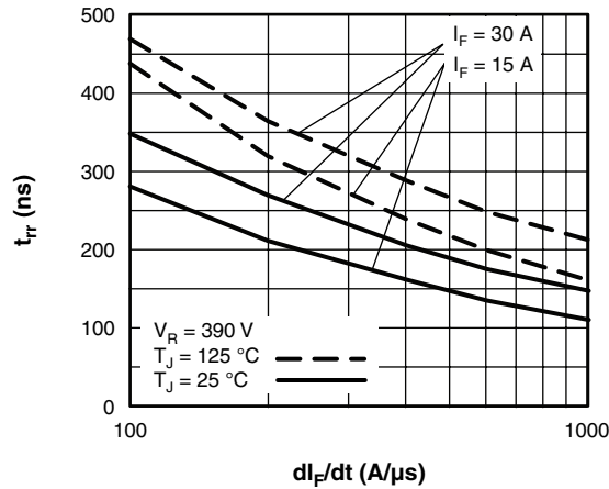
Fig. 9 - Typical Reverse Recovery Time vs. di_p/dt
