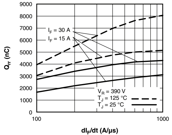
Fig. 10 - Typical Stored Charge vs. di_p/dt
